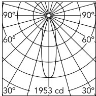
Luminous flux luminaire 722 lm (EXTREME CUT OFF)
